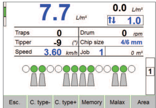
Dosing computer
